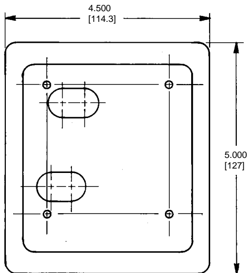
STANDARD MOUNTING BRACKET
