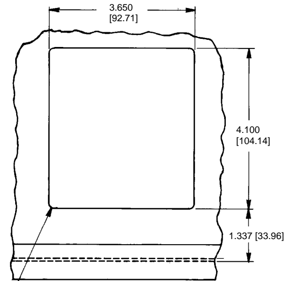
CUTOUT AND DOOR EDGE DETAIL FOR SINGLE POINT ASSEMBLY
