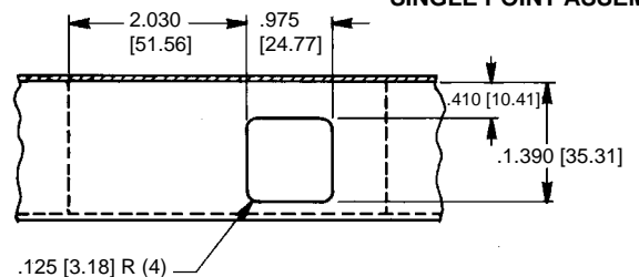
CUTOUT AND DOOR EDGE DETAIL FOR SINGLE POINT ASSEMBLY
